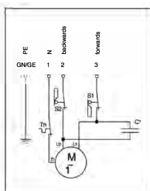
WS0800/230V 1AC
